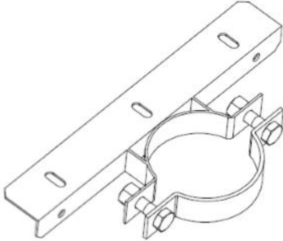
The Pole staple bolt 抱箍
